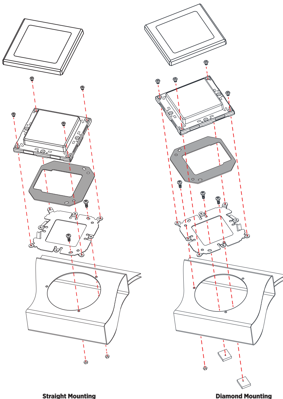
Straight Mounting
